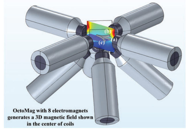
FIG. 2. A schematic of the OctoMag system 12 and the soft microrobot. The microrobot is steered by changes in the direction of the magnetic field. The microrobot dimensions are exaggerated to afford better visualization; the microrobot is illustrated in three different positions: (a) the initial position; (b) after deformation in the z direction; and (c) after deformation in the x direction. Color images are available online.
