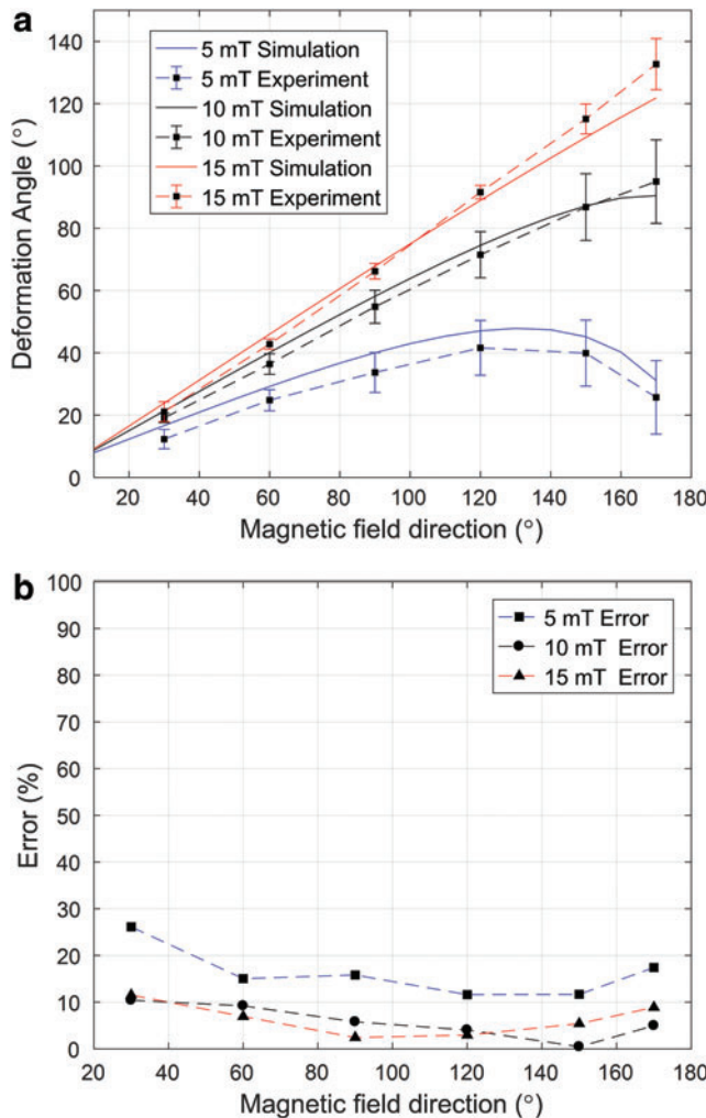
FIG. 7. Simulated and experimental deformation angles when the field directions varied ( n=3 for the experimental results). (a) Simulation (field directions between 10° and 170°) and experimental (field directions 30°, 60°, 90°, 120°, 150°, and 170°) results. (b) The differences between the experimental results and the simulations for field directions of 30°, 60°, 90°, 120°, 150°, and 170°. Color images are available online.
