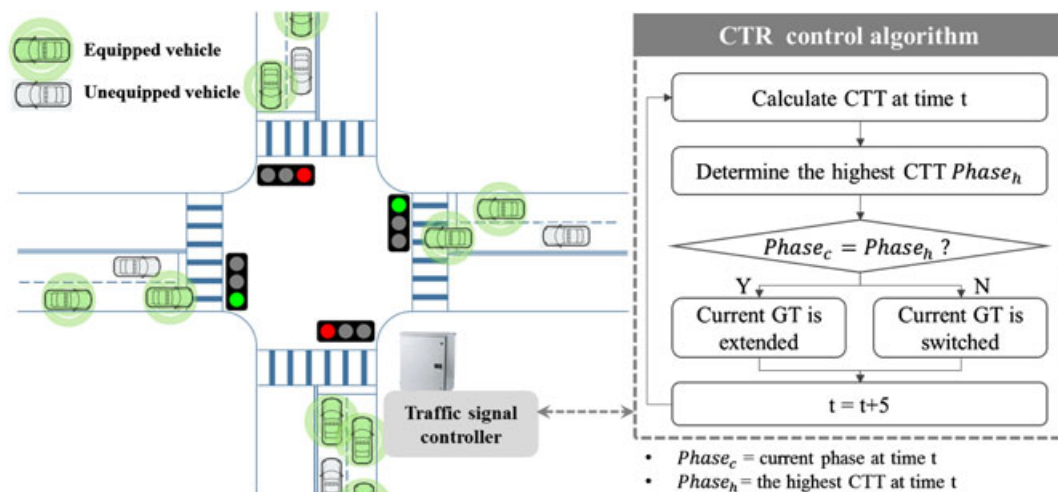
Figure 1. Concept of the cumulative travel-time responsive algorithm.
