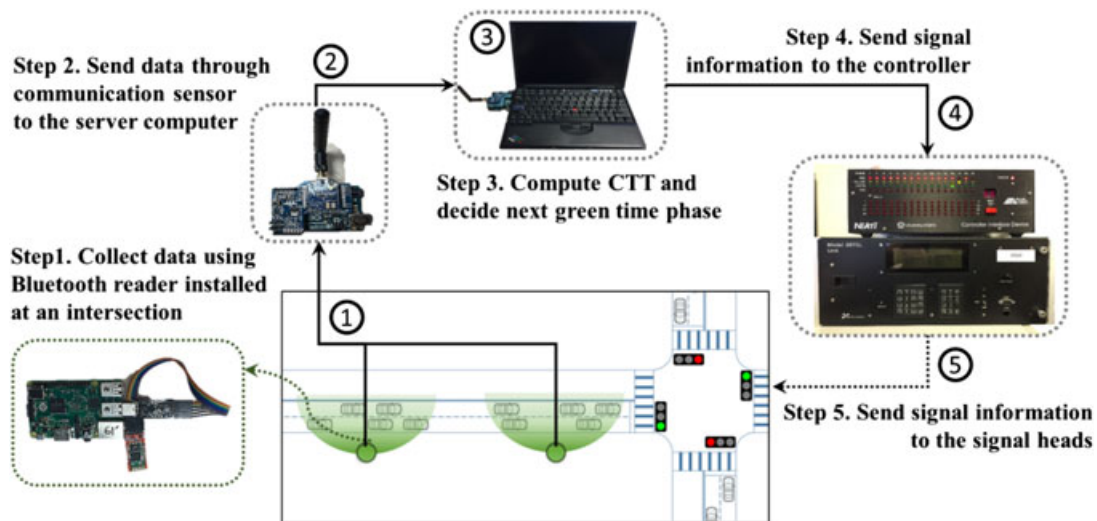
Figure 4. Hardware in the loop simulation configuration for the cumulative travel-time responsive algorithm.
