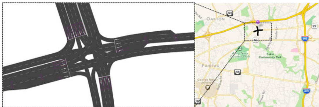
Figure 2. VISSIM network for study area.
