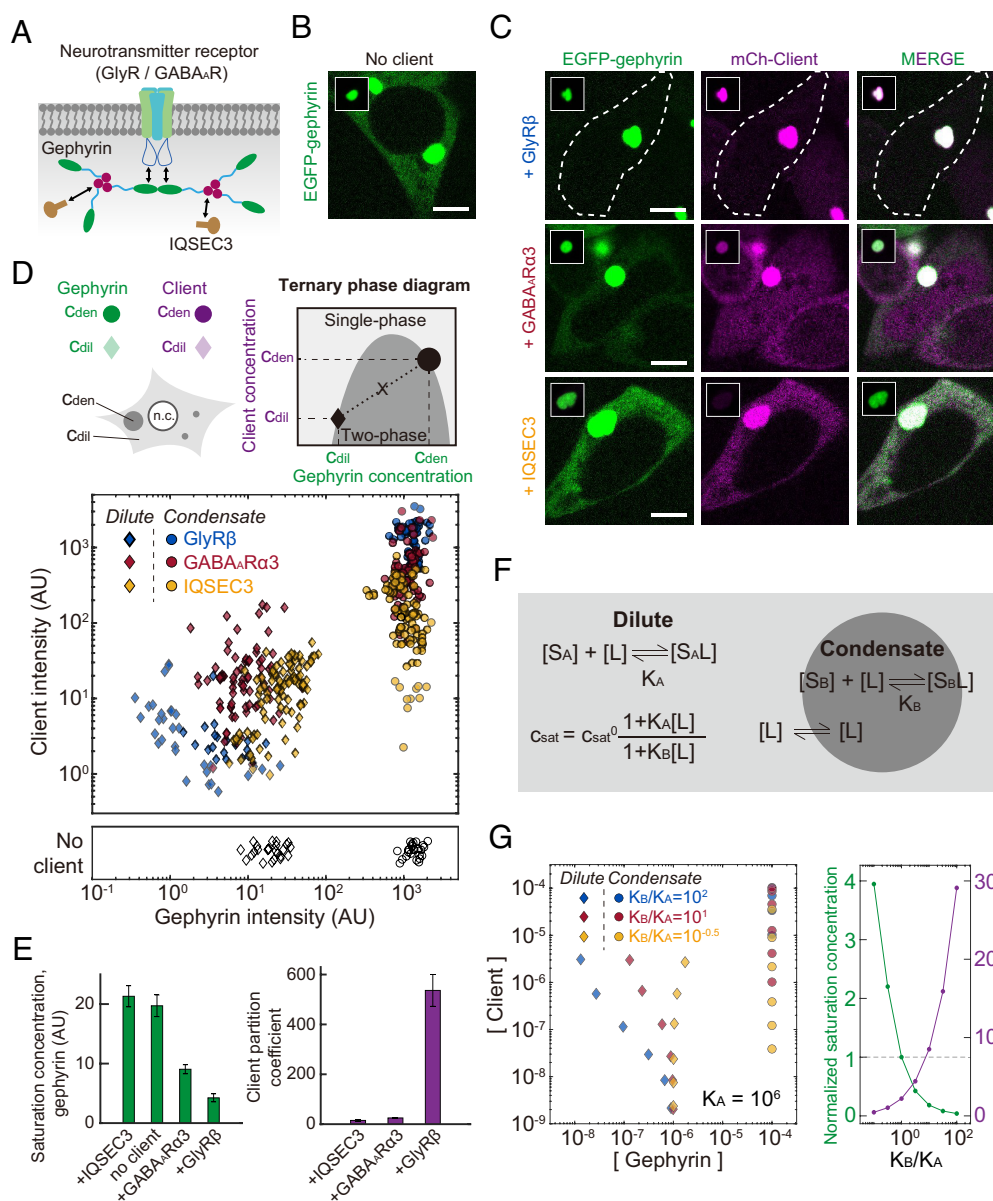
Fig. 6. iPSD components thermodynamically modulate gephyrin phase separation. (A) Schematic diagram of iPSD components used in this study and intermolecular interactions between them. (B and C) Fluorescence images of HEK293T cells expressing EGFP-tagged gephyrin WT alone (B) or coexpressing EGFP-tagged gephyrin and mCh-tagged iPSD components (C). Gephyrin and iPSD component expression levels are similar across these cells. For comparison, images are shown at the same brightness level. White dotted lines indicate cell boundary. Insets display gephyrin condensates in individual cells. Note that different brightness levels are used between the whole-cell images and insets. (Scale bars, 6 \mu m.) (D) (Top) Schematic diagram of the ternary phase diagram for gephyrin and iPSD components. Fluorescence intensities of molecules inside and outside of condensates constitute right- and left-hand boundaries of the two-phase region, respectively. (Bottom) Experimentally measured ternary phase diagram of gephyrin and individual iPSD components. The concentrations of the dilute- and dense phase were measured for cells containing gephyrin condensates. Data acquired with gephyrin alone are shown for comparison. Imaging conditions used in this analysis are different from those in the characterization of saturation concentrations of various gephyrin variants shown in Figs. 1–3. GlyR- \beta , n = 52 ; GABA A R- \alpha 3 , n = 73 ; IQSEC3, n = 88 ; no client, n = 25 . (E) Saturation concentration of gephyrin in the presence or absence of specific iPSD components (Left). Partition coefficients of iPSD components, defined as a ratio of the concentration inside gephyrin condensates versus the surrounding cytoplasm (Right). Cells with similar expression levels are used in these quantifications. Error bars \pm SEM; GlyR- \beta , n = 37 ; GABA A R- \alpha 3 , n = 42 ; IQSEC3, n = 27 ; gephyrin alone, n = 17 . (F) Schematic diagram of the polyphasic linkage model. Preferential binding of clients to scaffolds in one phase over the other leads to a change in scaffold saturation concentration (SI Appendix). In each phase, clients exhibit equilibrium binding to scaffolds, characterized by an association constant K_i . (G) (Left) Predicted ternary phase diagrams based on the polyphasic linkage model ( K_A = 10^6 M -1 ). To generate the diagrams, six different pairs of total gephyrin/client concentrations are used for each condition (Materials and Methods). All concentrations are in molarity. (Right) Changes of normalized saturation concentration and client partition coefficient by preferential binding effects. Results are obtained from model calculation using the identical total concentrations of scaffolds and clients.
