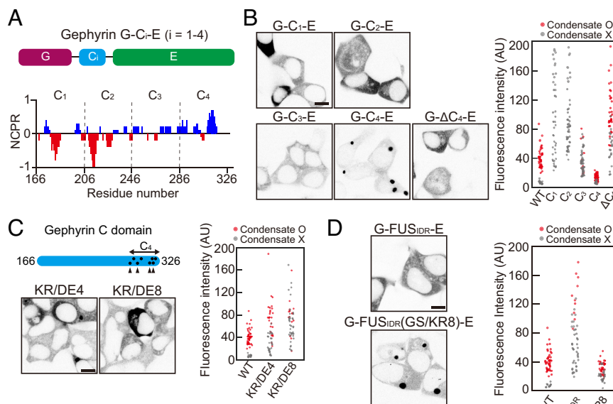
Fig. 3. The positive charges near the C-terminal end of the C domain are important for phase separation. (A) Schematic of gephyrin variants with C-domain truncation. Net charge per residue plot of the gephyrin C domain, calculated with a sliding window of 5 residues. (B) (Left) Fluorescence images of EGFP-tagged gephyrin variants with different C-domain truncation or C 4 deletion in HEK293T cells. (Scale bar, 8 μm.) (Right) Cytosolic fluorescence intensity of HEK293T cells expressing gephyrin WT or variants with different C-domain truncations or C 4 deletion. (C) (Top Left) Schematic of gephyrin variants with positively charged residues mutated into negatively charged ones (KR/DE4 and KR/DE8). Dots indicate positively charged residues in the C 4 subregion mutated in KR/DE8, and arrowheads denote the locations of mutated residues in both KR/DE4 and KR/DE8. (Bottom Left) Fluorescence images of gephyrin variants, KR/DE4 and KR/DE8 in HEK293T cells. (Scale bar, 8 μm.) (Right) Cytosolic fluorescence intensity of HEK293T cells expressing gephyrin WT or variants. (D) (Left) Fluorescence images of EGFP-tagged G-FUS IDR -E and G-FUS IDR (GS/KR8)-E in HEK293T cells. (Scale bar, 8 μm.) (Right) Cytosolic fluorescence intensity of HEK293T cells expressing gephyrin WT or variants.
