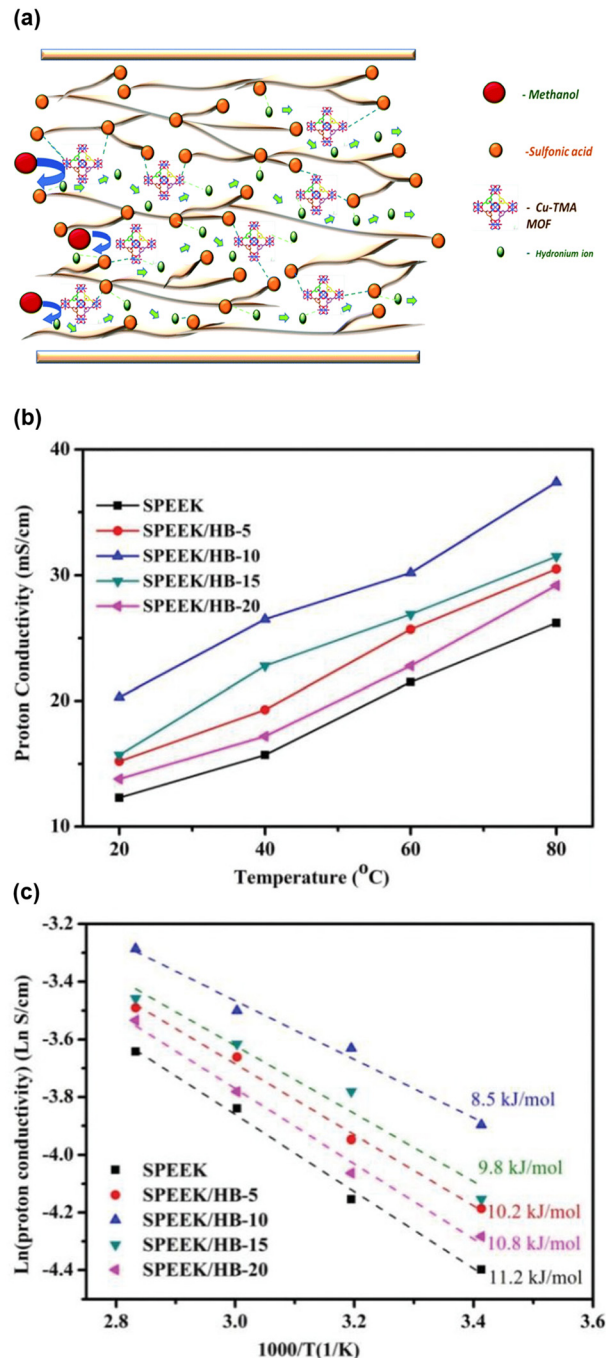
Fig. 11 (a) Illustration of HKUST-1 in sSPEEK matrix, SP/CT-MOF-3, depicting hydrogen bond network, proton transport pathways and low methanol permeability. Reproduced with permission from ref. 100, Copyright 2018, Royal Society of Chemistry. (b) Proton conductivity and (c) Arrhenius plots of pristine SPEEK and HKUST-1/ \text{BPO}_4 in sSPEEK matrix. Reproduced with permission from ref. 101, Copyright 2021, Wiley VCH.
