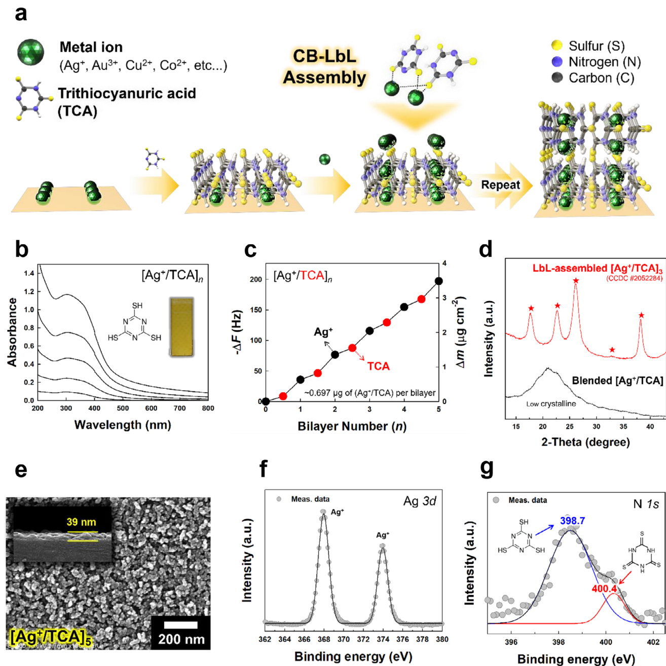
Figure 2. LbL-assembled MOF multilayers. a) Schematic illustration for the preparation of LbL-assembled [Ag + /TCA] n multilayers onto Ni-ET. b) UV-vis spectra and c) QCM data of [Ag + /TCA] n multilayers with different bilayer numbers ( n ). Insets in Figure 2b show the molecular structure of TCA and a digital image of [Ag + /TCA] n multilayer-coated quartz substrate. d) XRD patterns of LbL-assembled [Ag + /TCA] 3 multilayers and blended Ag + -TCA films. e) FE-SEM image of [Ag + /TCA] 5 multilayers onto Si wafer. The inset shows the cross-sectional FE-SEM image of [Ag + /TCA] 5 multilayers. f) Ag 3d and g) N 1s XPS spectra of [Ag + /TCA] 5 -MOF multilayers. Deconvolution of the N 1s spectrum reveals the presence of two types of molecular structures of TCA within the [Ag + /TCA] 5 -MOF multilayers.
