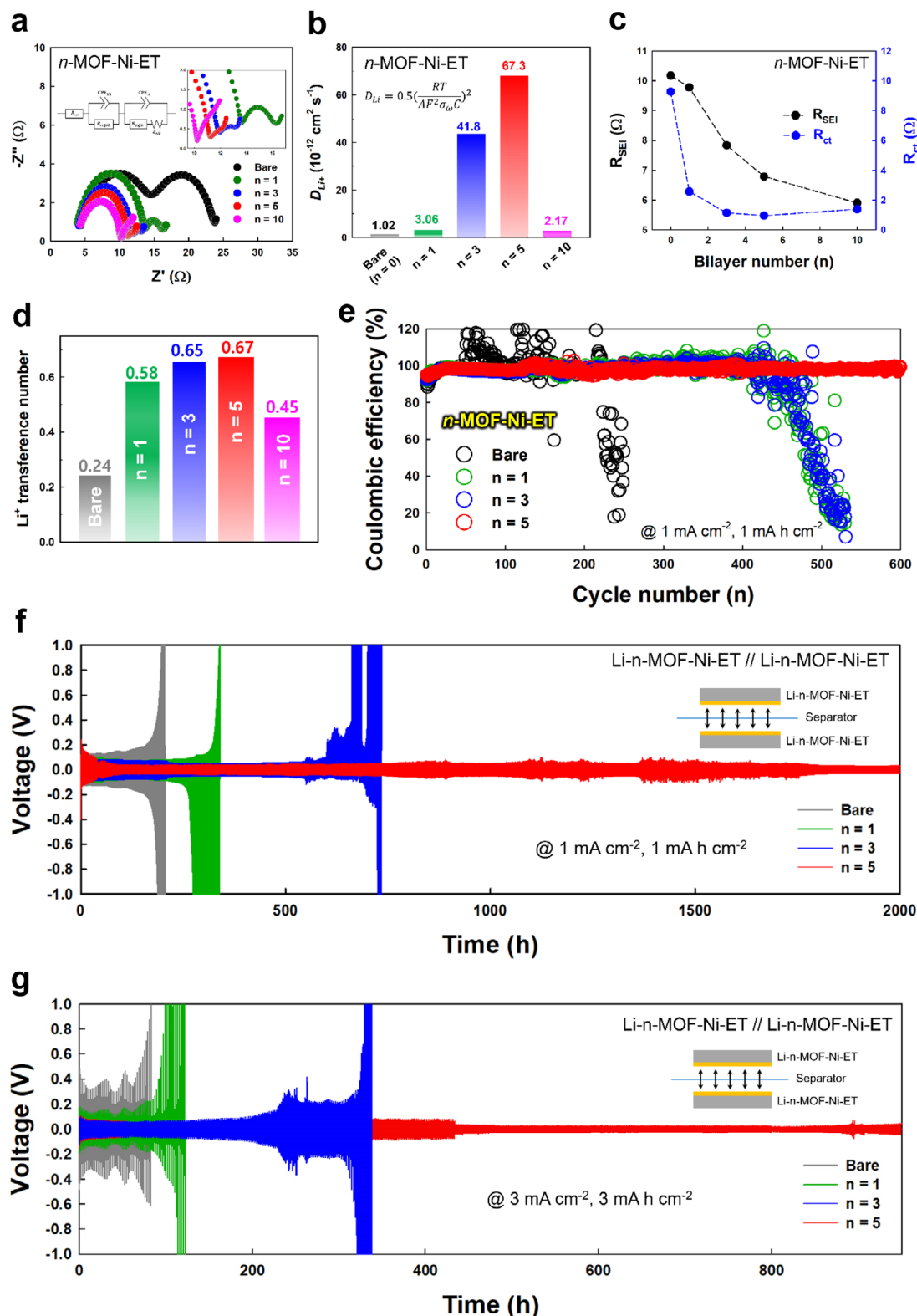
Figure 4. Symmetric cell tests. a) Nyquist plots of \text{Li//Li-}n\text{-MOF-Ni-ET} half-cells as a function of bilayer number ( n ) of 0, 1, 3, and 5. Inset shows enlarged impedance spectra in the low-frequency region and the representative equivalent circuit. b) Ion diffusion coefficients ( D_{\text{Li}^+} ), and c) R_{\text{SEI}} and R_{\text{ct}} values of \text{Li//Li-}n\text{-MOF-Ni-ET} half-cells as a function of bilayer number ( n ). d) \text{Li}^+ transference number of \text{Li//Li-}n\text{-MOF-Ni-ET} half-cells as a function of bilayer number ( n ). e) CE values of \text{Li//Li-}n\text{-MOF-Ni-ET} half-cells during Li plating/stripping cycles at 1 \text{ mA cm}^{-2} and 1 \text{ mA h cm}^{-2} . Galvanostatic cycling of bare Ni-ET and n\text{-MOF-Ni-ET} -based symmetrical full-cells at f) 1 \text{ mA cm}^{-2} ( 1 \text{ mA h cm}^{-2} ) and g) 3 \text{ mA cm}^{-2} ( 3 \text{ mA h cm}^{-2} ).
