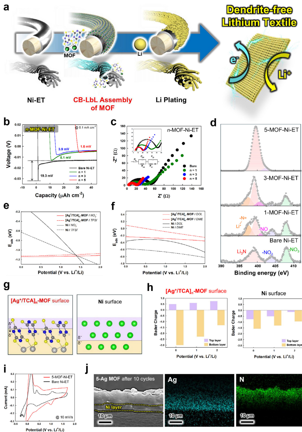
Figure 3. Li textile node. a) Schematic illustration for the preparation of LTA. b) Voltage (V) versus capacity ( \mu Ah\ cm^{-2} ) curves of bare Ni-ET and n -MOF-Ni-ET-based half-cells during Li nucleation at 0.1\ mA\ cm^{-2} and 6\ mAh\ cm^{-2} . c) Nyquist plots of bare Ni-ET and n -MOF-Ni-ET half-cells. Insets show enlarged impedance curves in the high-frequency region and the representative equivalent circuit. d) N 1s XPS spectra of bare Ni-ET and n -MOF-Ni-ETs with different bilayer numbers ( n ). e) Calculated anion adsorption energy ( E_{ads} ) versus potential curves of anion molecules ( NO_3^- and TFSI^- ) and f) solvent molecules (DME and DOL) adsorbed onto bare Ni-ET and n -MOF-Ni-ET electrodes. g) Schematic illustration of surface configurations for bare Ni-ET and n -MOF-Ni-ET surfaces. h) Bader charge analysis of bare Ni and [Ag^+/TCA]_n -MOF surfaces at different potentials. i) Cyclic voltammograms of bare Ni-ET and 5-MOF-Ni-ET electrodes at a scan rate of 10\ mV\ s^{-1} . j) Cross-sectional FE-SEM image and corresponding elemental mapping images (Ag and N) of the 5-MOF-Ni-ET electrode after 10 cycles.
