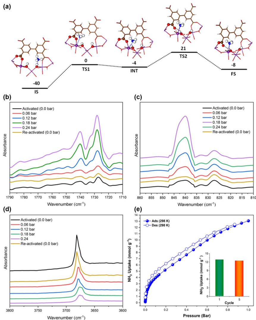
Fig. 27 (a) DFT-simulated potential energy profile for \text{NH}_3 -triggered Sc-coxycylate dynamic bonding in MFM-300(Sc), showing the initial state (IS), transition states (TS1 and TS2), intermediate (INT), and final state (FS). Color code: C (brown), O (red), N (blue), H (white), and Sc (purple); energies in \text{kJ mol}^{-1} . (b–d) DRIFTS of \text{NH}_3 dosed over activated MFM-300(Sc) at 298 K and 0–0.24 bar, shown for (b) 1790–1710 \text{cm}^{-1} , (c) 860–810 \text{cm}^{-1} , and (d) 3800–3600 \text{cm}^{-1} regions. (e) \text{NH}_3 adsorption (filled blue) and desorption (open blue) isotherms at 298 K up to 1 bar; inset compares uptake in the 1st and 5th cycles. Reproduced with permission from ref. 29, Copyright 2021, American Chemical Society.
